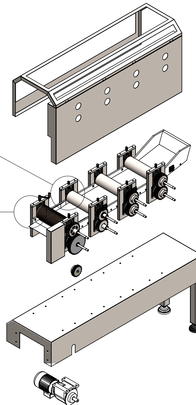
EXPLODED VIEW OF EQUIPMENT SUPPLIED SCALE 1:20
